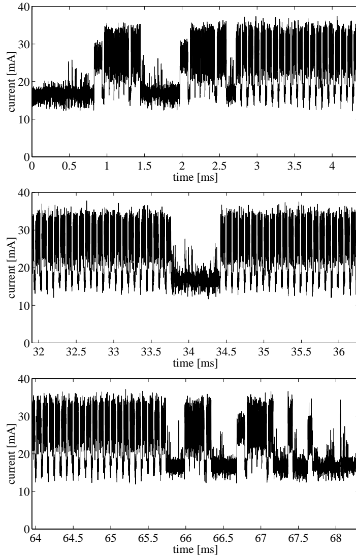
Fig. 1. Typical power consumption patterns during RSA decryption
