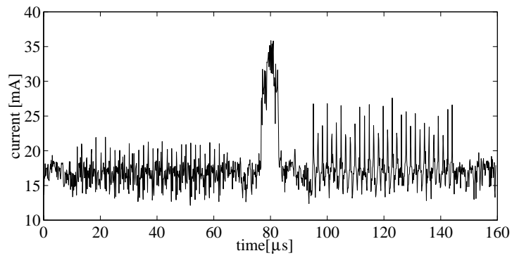
Fig. 3. Detailed view of optional pattern
