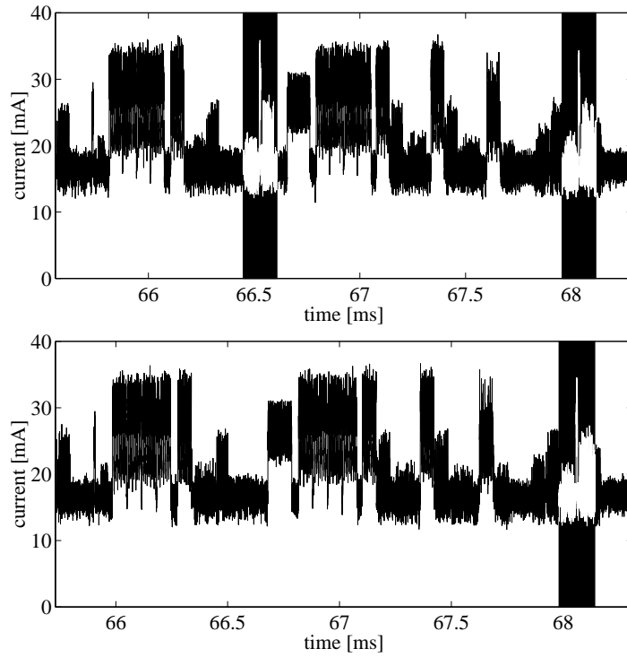
Fig. 2. Two types of power trace tails
